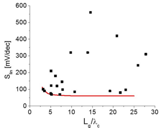
FIGURE 11. Linear subthreshold swing vs. ratio of gate length to electrostatic characteristic length of InGaAs VNW MOSFETs. For reference, the ideal electrostatic behavior is also indicated [62].
